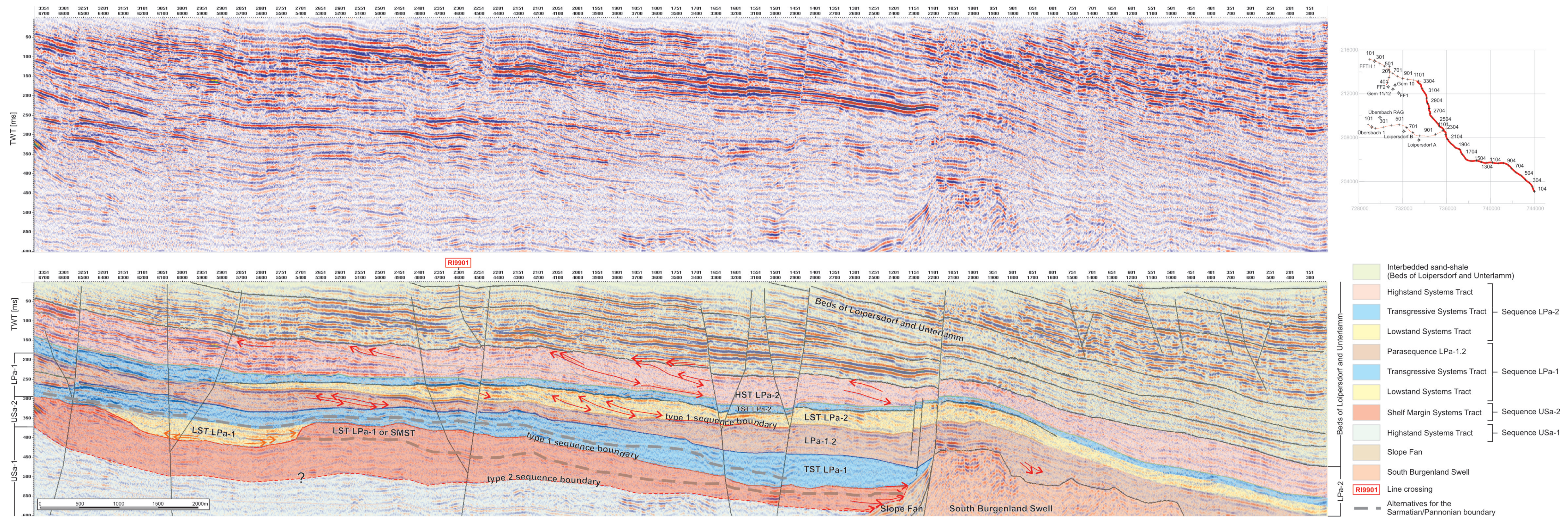
Fig. 4: Seismic line UL9901 and its interpretation. TWT – Two way travel time.
